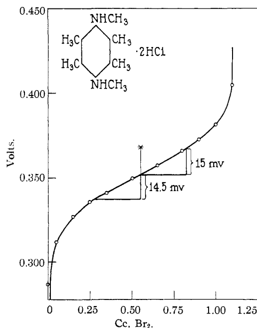
Fig. 2.—Symmetrical dimethyldurene diamine bihydrochloride. Conditions of titration the same as in Fig. 1. Here also a full titration curve is obtained. The index potential is between 14 and 15 mv., indicating that no intermediate radical is formed, in agreement with the fact that no trace of any intermediate colored compound is visible during the titration. The point * in this and all the other curves marks the end of the first step, where 1 atom of bromine per molecule of the diamine has been added.
